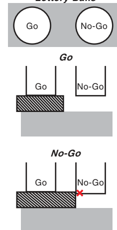
Go/No Go Gauge for Lottery Balls
