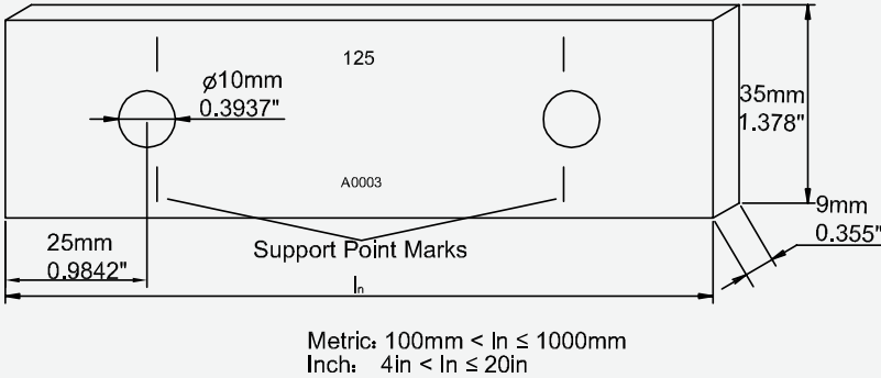
Gage Block Measurement Reference
