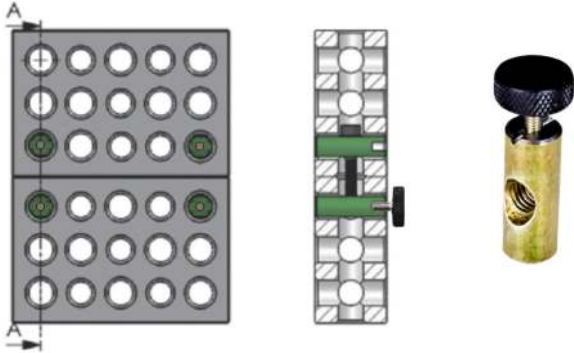
Using this hardware allows two blocks to be attached to each other in literally every possible configuration
