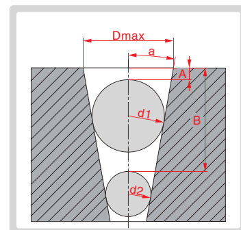
Calculate angle (a) and diameter (Dmax) according to the ball diameter (d1, d2), height (A) and depth (B)
